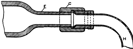
FIG. 185.—Diagram of the Haythorn joint used on the Simpson-Bodman and other flash generators.
